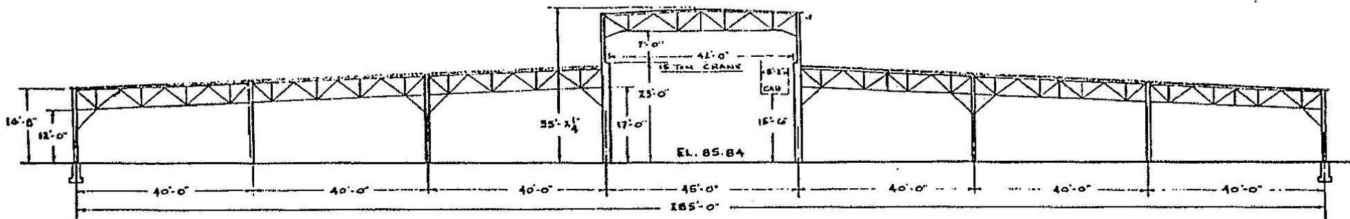
CROSS SECTION BLDG. #1
