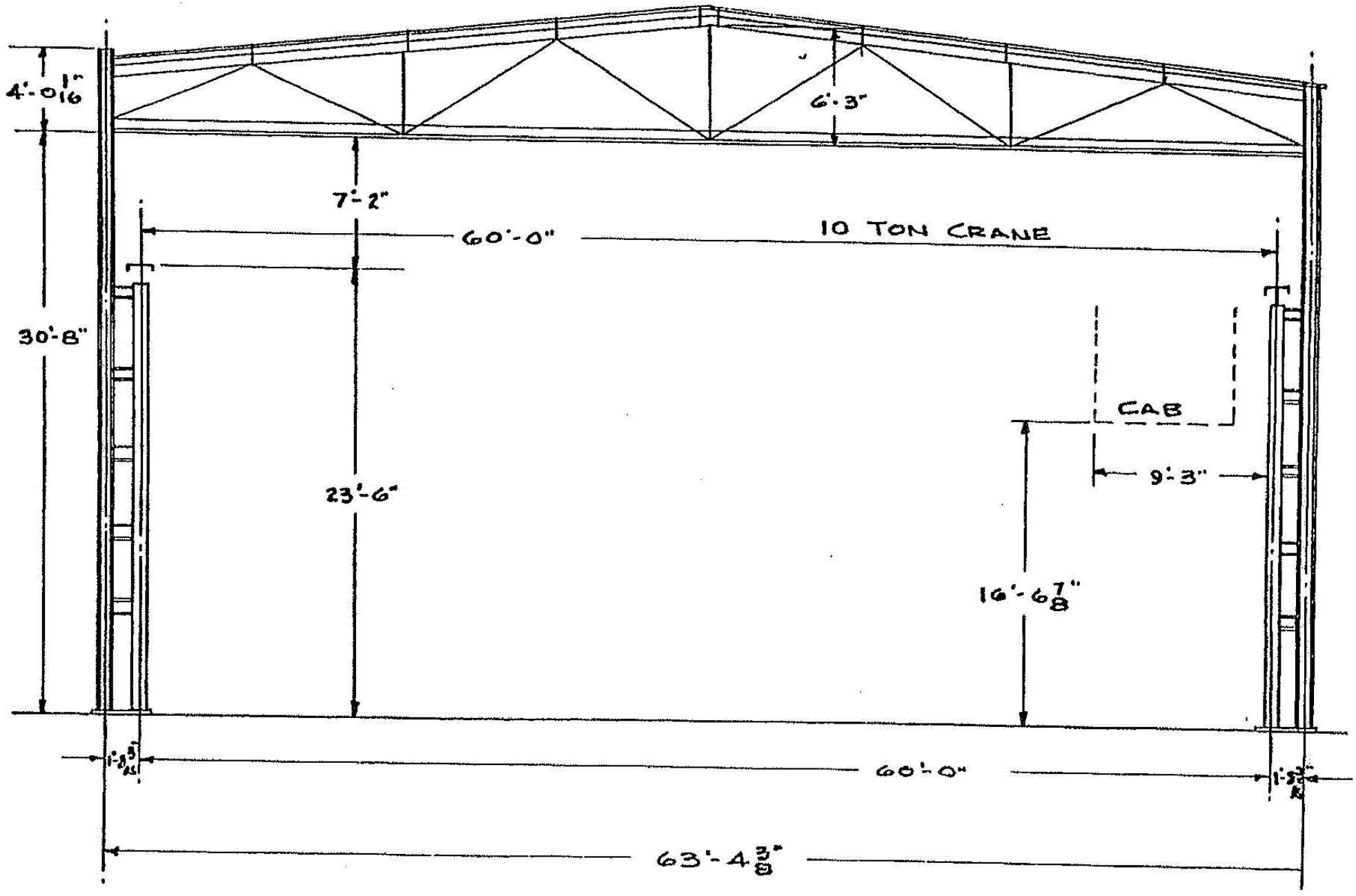
CROSS SECTION BLDG. # 35
