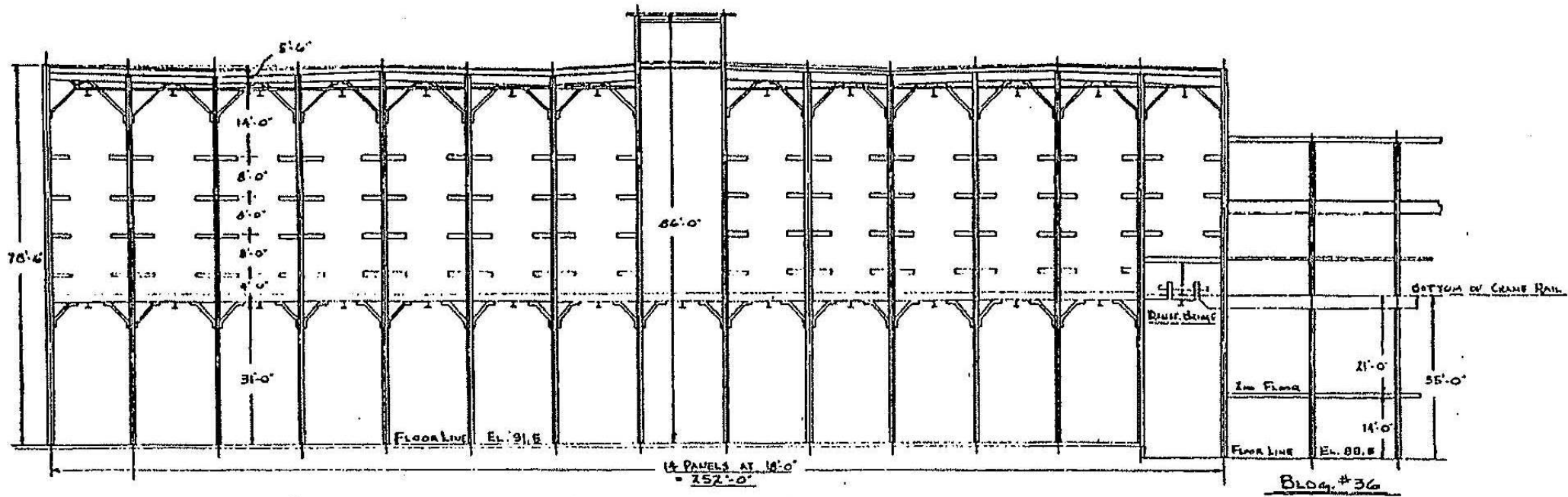
CROSS SECTION BLDG. #36
