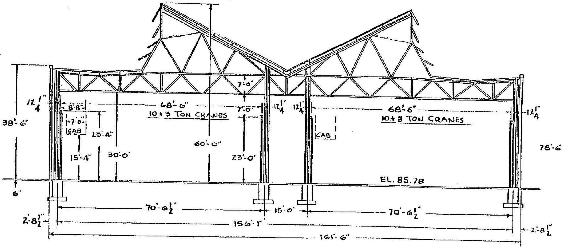
CROSS SECTION BLDG # 52
