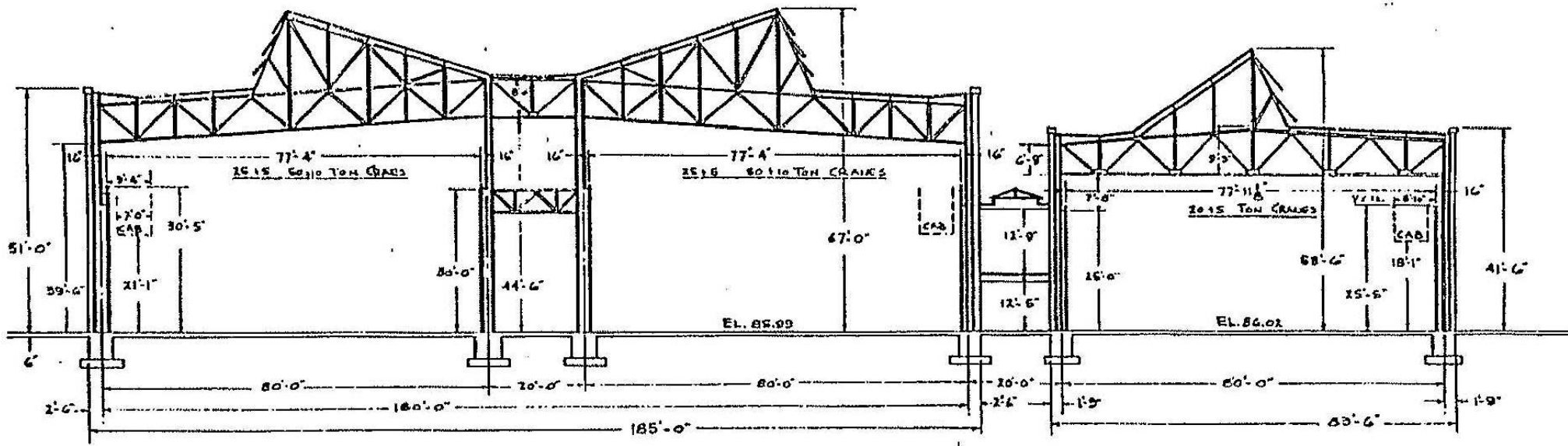
CROSS SECTION Bldg. # 51
